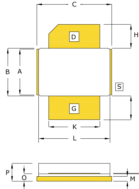
EARLESS FLANGE OPTION IGN2731M1700S
