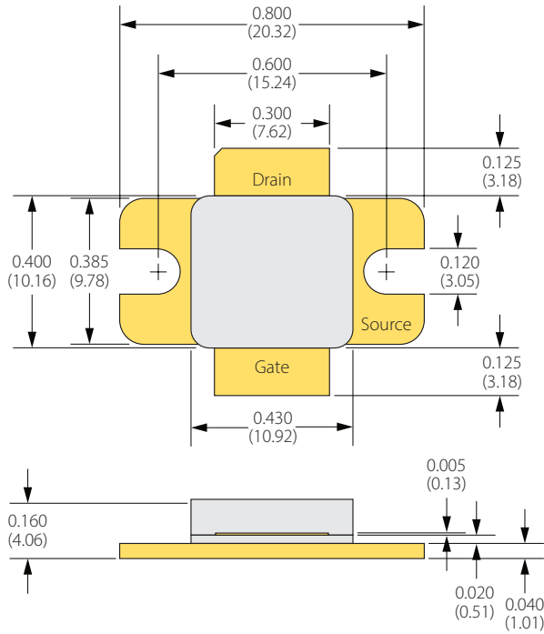
BOLT-DOWN FLANGE OPTION IGN1011L120
