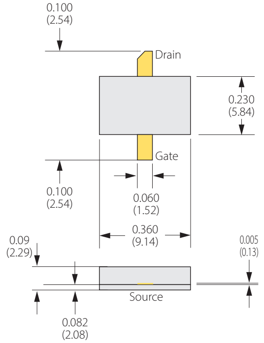
EARLESS FLANGE OPTION IGN1011L60S
