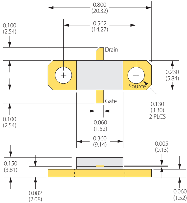
BOLT-DOWN FLANGE OPTION IGN1011L60
